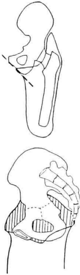
Fig. 3. UCLA CAT-CAM. Top, ischial inclination angle. Bottom, medial view of pelvis-socket relationship.
