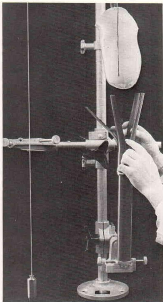
Fig. 13. Use of a PVC tube as a supporting structure (shank) for a below-knee prosthesis.
