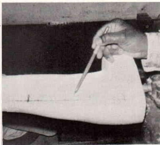
Fig. 17. Suction-socket valve installation in an AK prosthesis with a Cordo liner.
