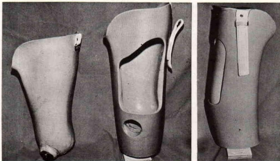
Fig. 16. Two-component type of total-contact AK suction socket designed for geriatric AK amputees. Left , flexible inner socket; center , rigid outer shell with anterior window; right , complete assembly of socket and shell held together by Velcro strap on lateral side.
