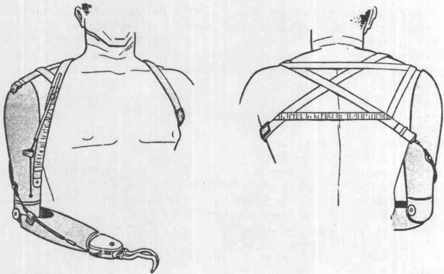
Fig. 1. One Version of the Figure-8 Harness for Above-Elbow Amputees
